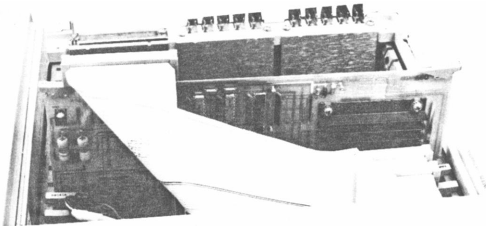
Figure 2-1. Installation of the HP 64501A PROM Programmer Control Board
